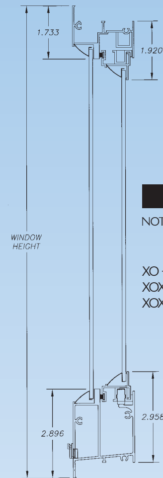
HORIZONTAL ROLLER FLANGE SERIES 201 SIDE VIEW DETAIL
