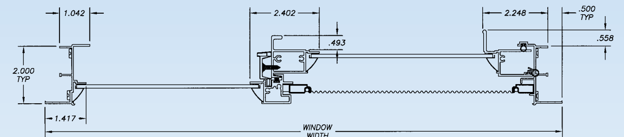
HORIZONTAL ROLLER FLANGE SERIES 201 TOP VIEW DETAIL
